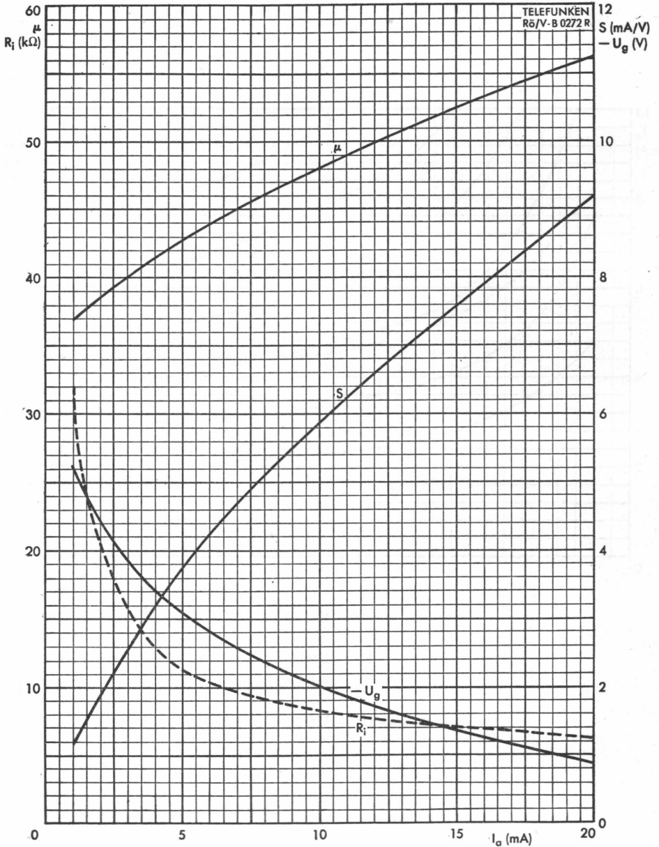
S, R_i, \mu, -U_g = f(I_a) U_a = 200 V
